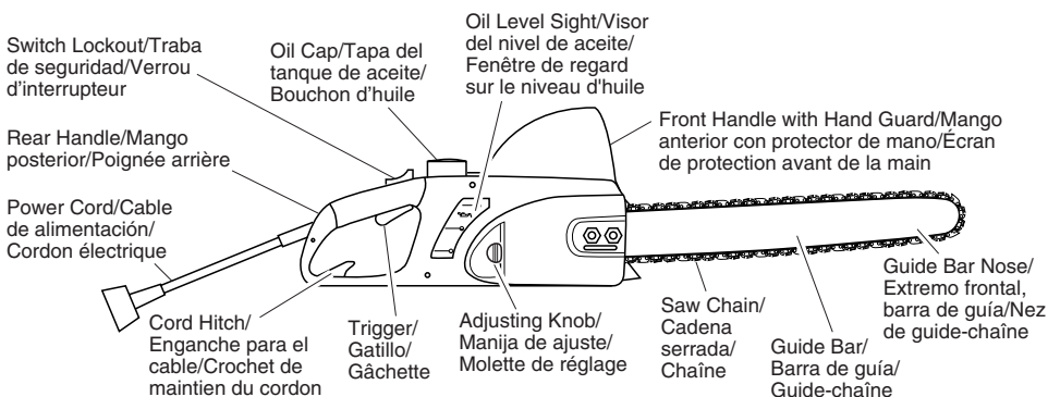
Figure 2 - Chain Saw Model 107625-01, -02
